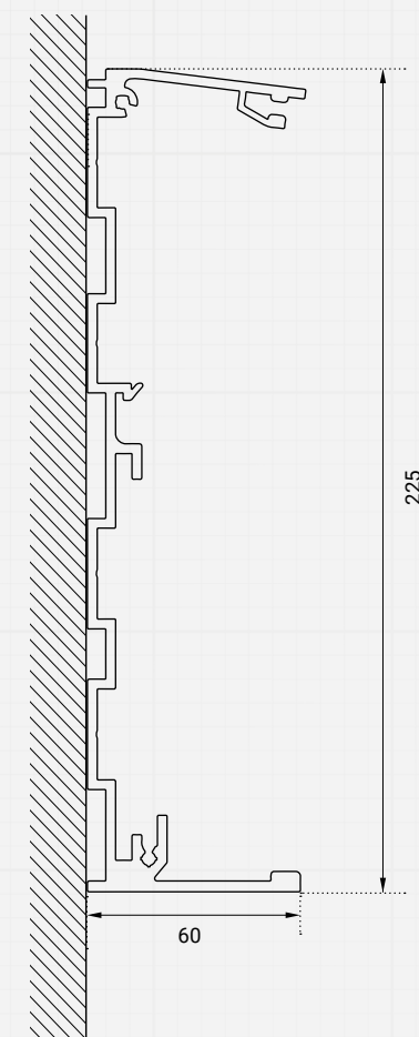
Wandprofil TR20 (Wandmontage)
